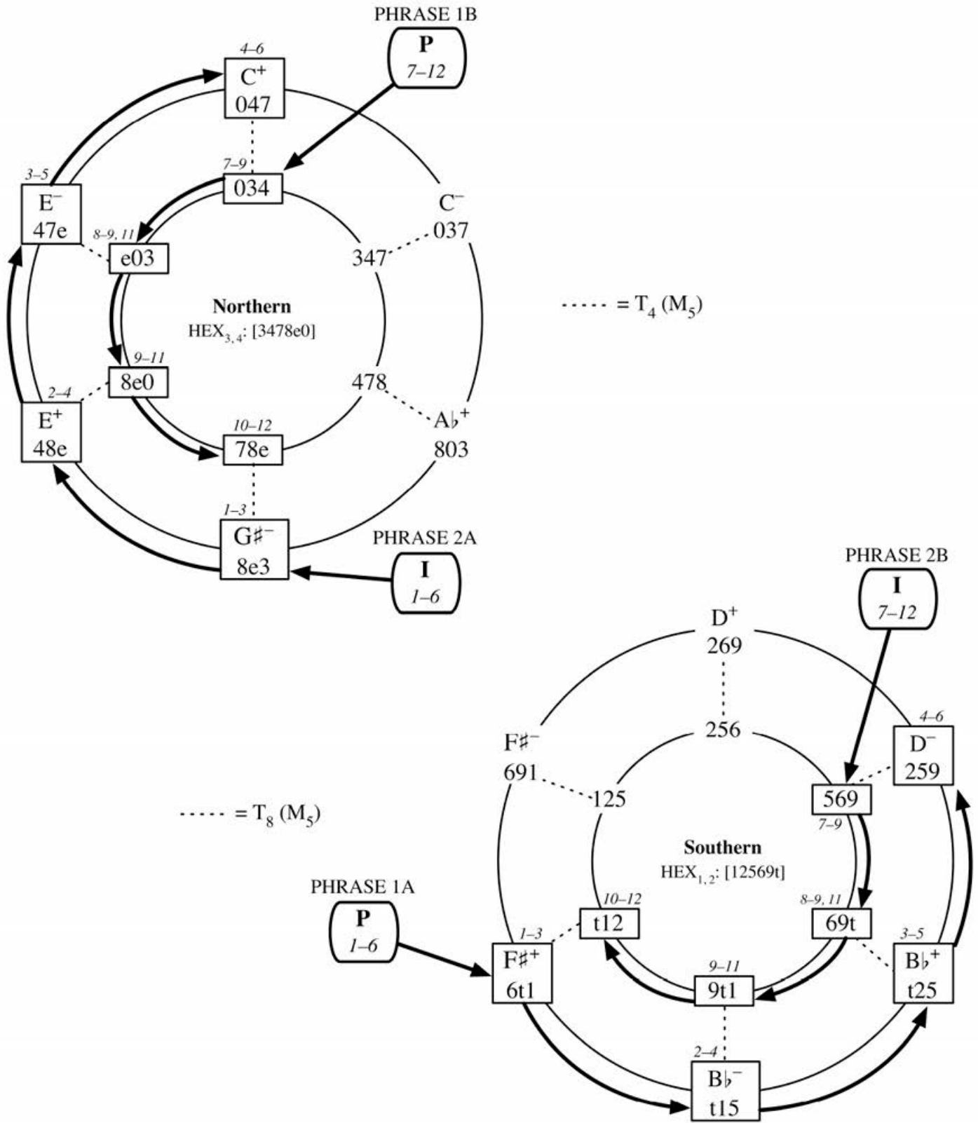
Example 1. Joseph Straus's visualization of triads and (014)s plotted on Richard Cohn's Northern and Southern hexatonic systems
